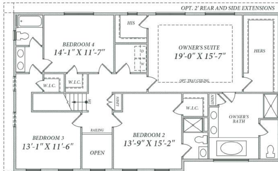
ALTERNATE SECOND FLOOR PLAN
